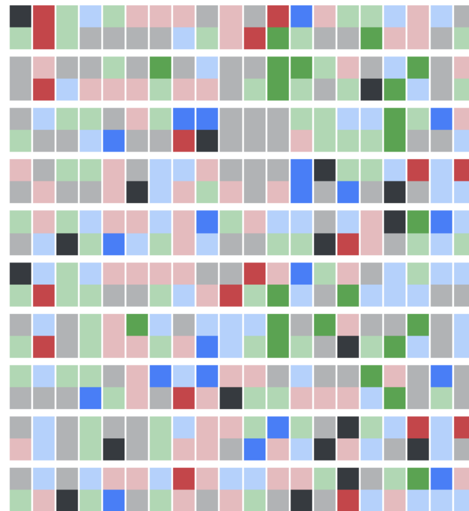
Imputed Genotypes
