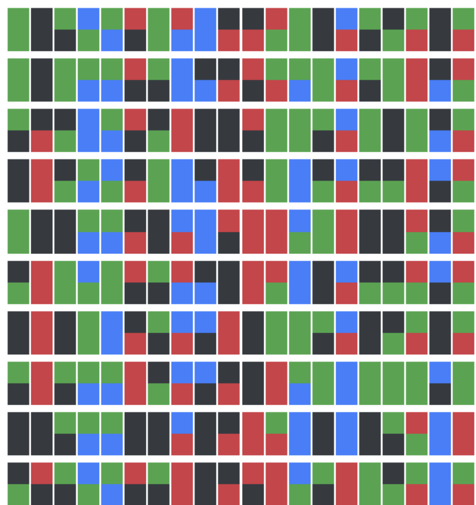
Reference Panel
