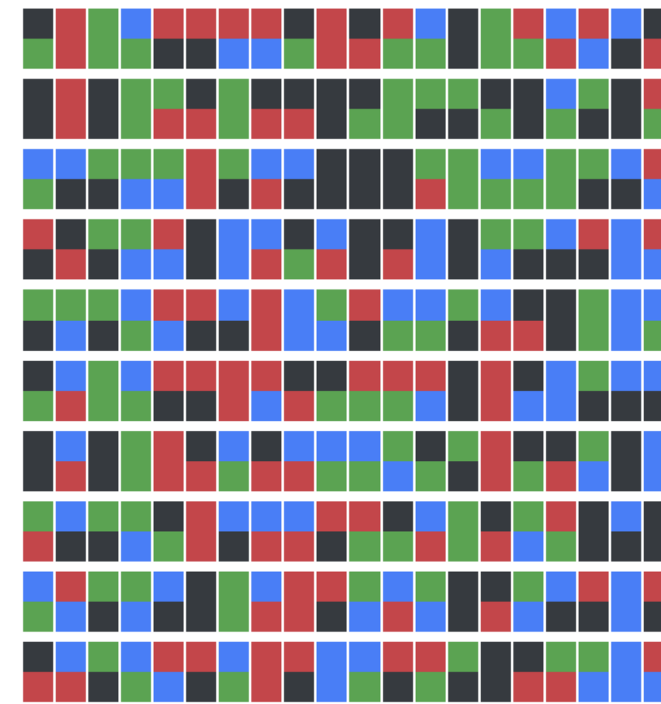
Sequenced to high coverage (30X)
