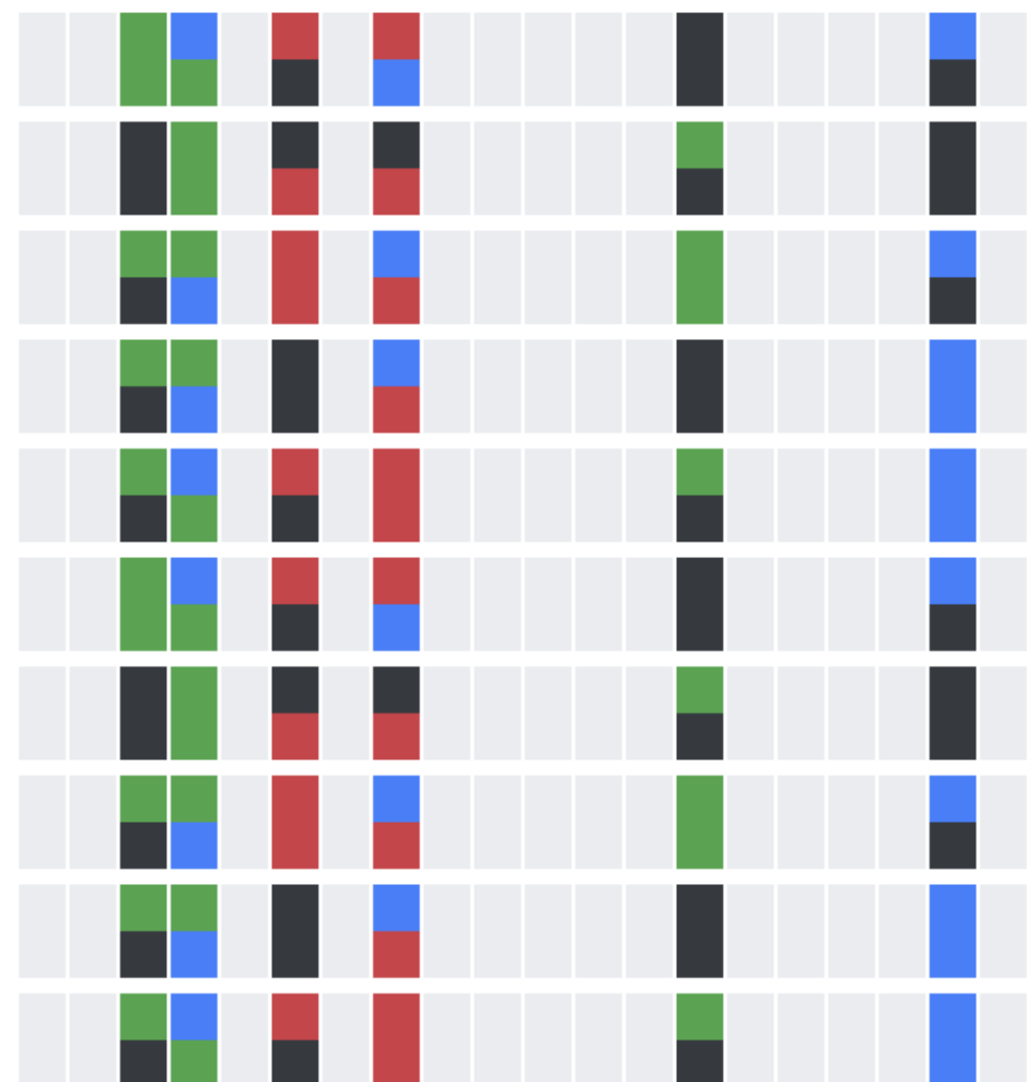
SNP Chip
