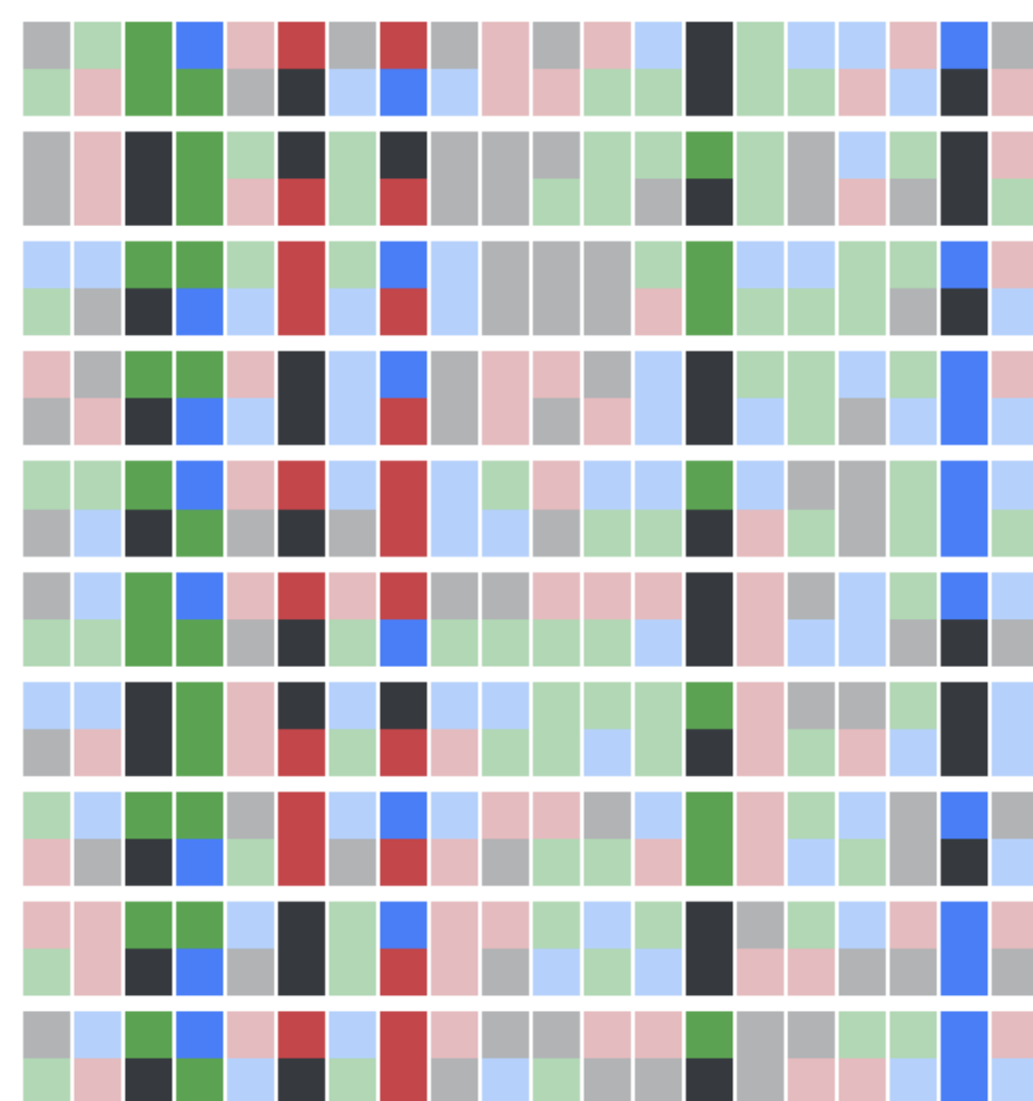
Imputed Genotypes
